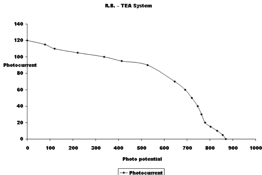
Figure 6: Current-potential (i-V curve) of the Rose Bengal- TEA cell systems
